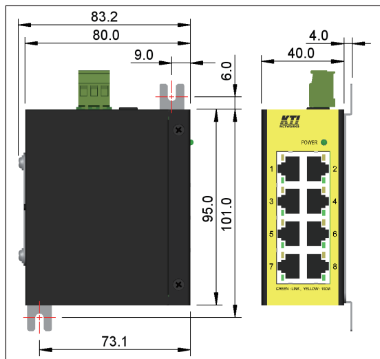
Panel & Wall Mount Dimension
