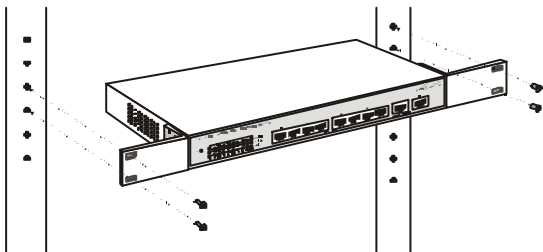
Figure 2-2B. Installing the Switch in an equipment rack
