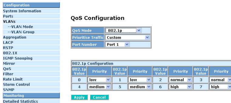
Fig. 4-22 802.1p Setting
