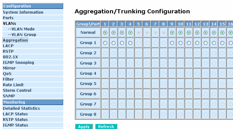
Fig. 4-10 Aggregation/Trunking Configuration
