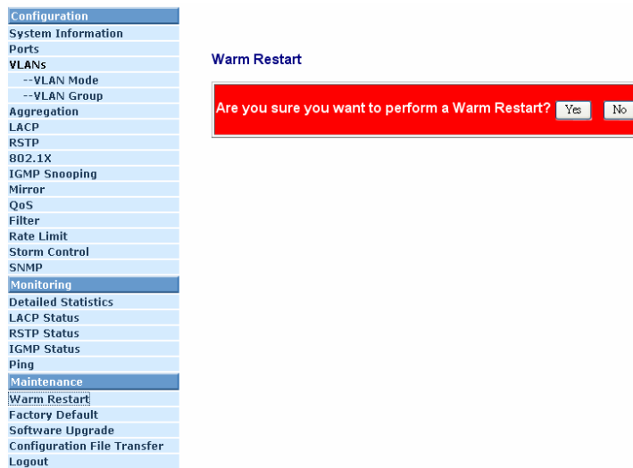
Fig. 4-34 Warm Restart
