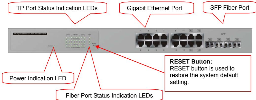
Fig. 1-2 Front View of 16-Port GbE Web Smart Switch
