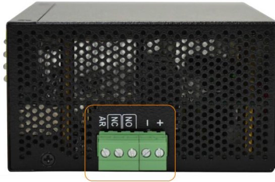
DC IN terminal block connector
