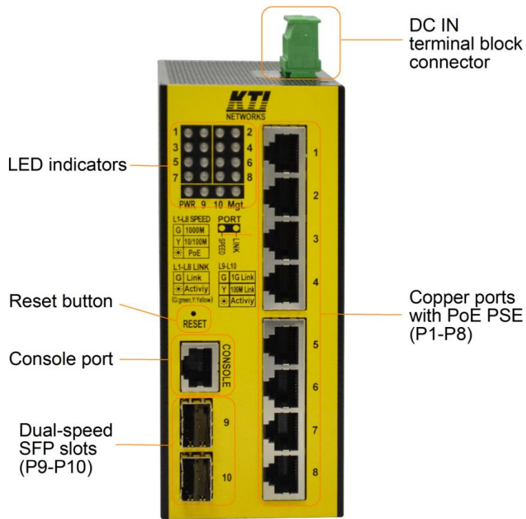
Front panel
