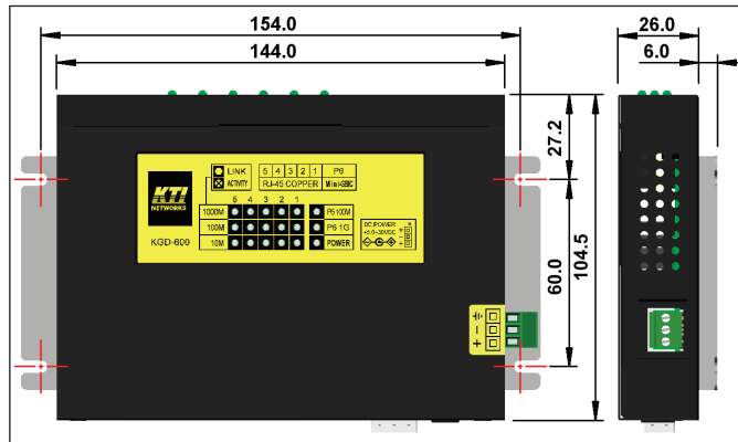
Panel & Wall Mount Dimension
