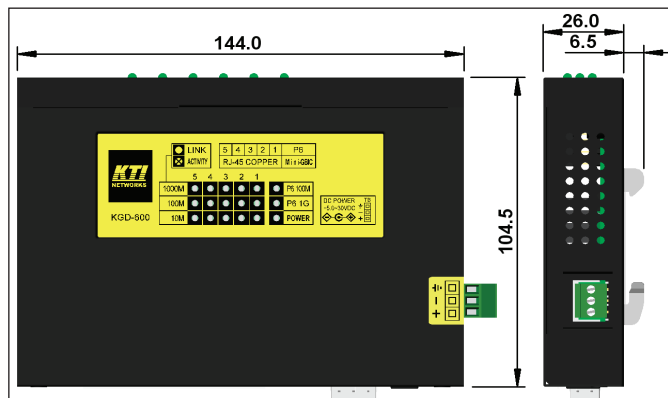
Din-Rail Mount Dimension
