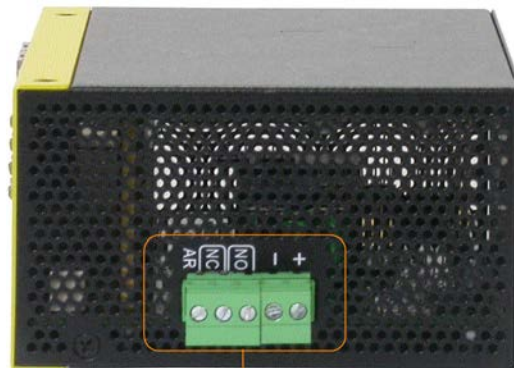
Terminal block connector
