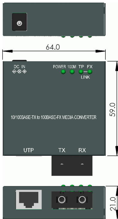
Media Converter with duplex SC connector
