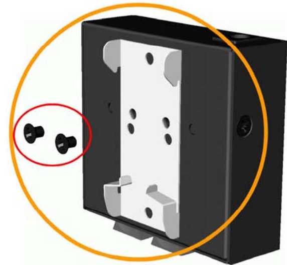
Din-Rail Mounting
