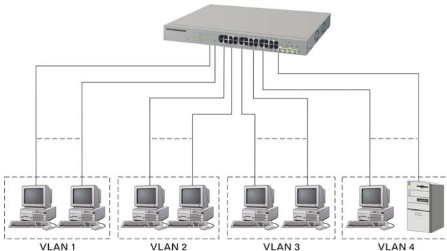
Fig. 2-3 Port-based VLAN Diagram
