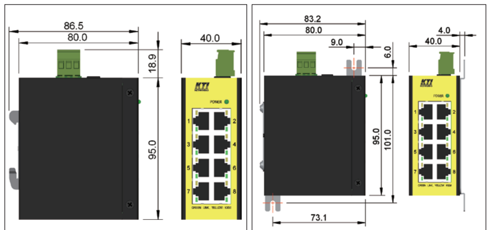
DIN-Rail Dimension
