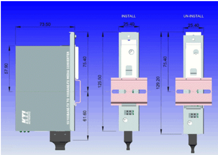
Figure B. KC-3DR Bracket
