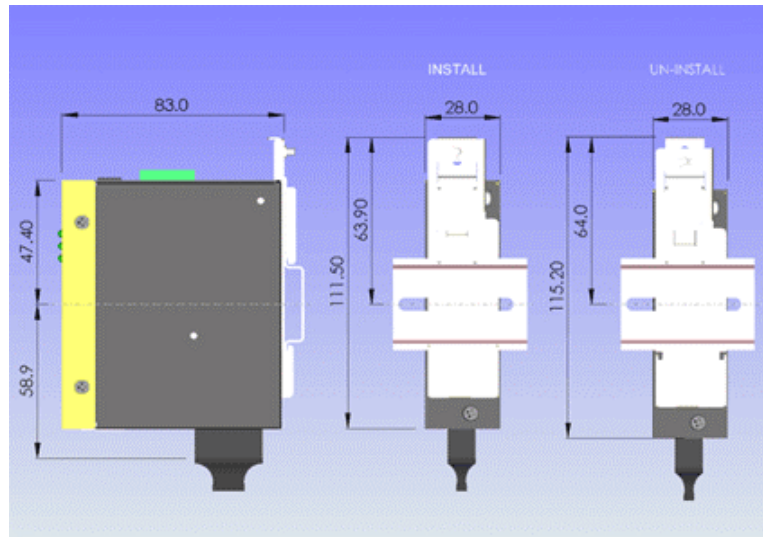
Figure C. Standard bracket for KCD-300 series
