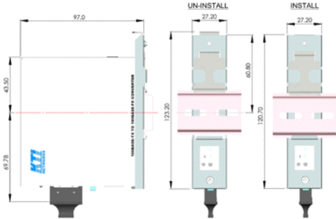
Figure A. KC-2DR Bracket
